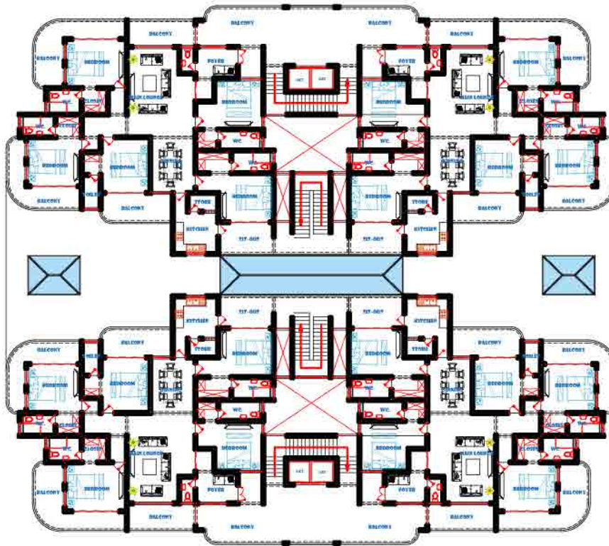
5 BEDROOMS BLOCK LAST FLOOR ON 2&1 BEDROOM BLOCK
